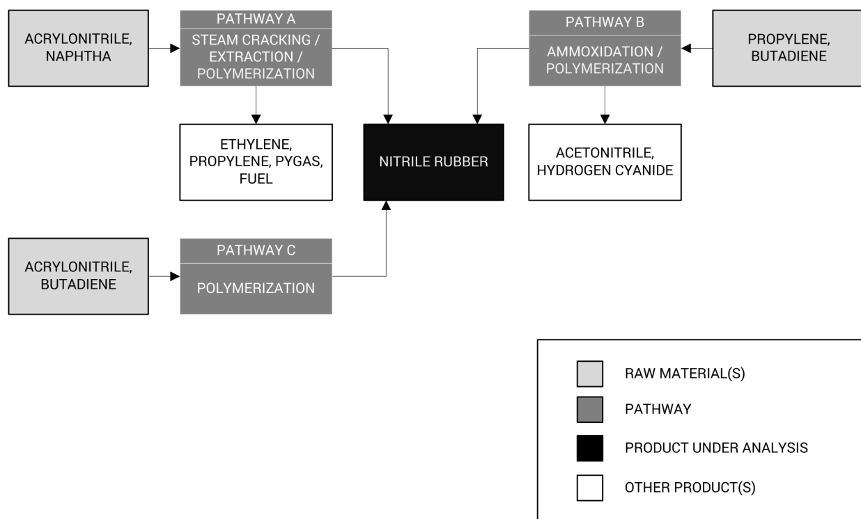
Nitrile Rubber Production Pathways Diagram
