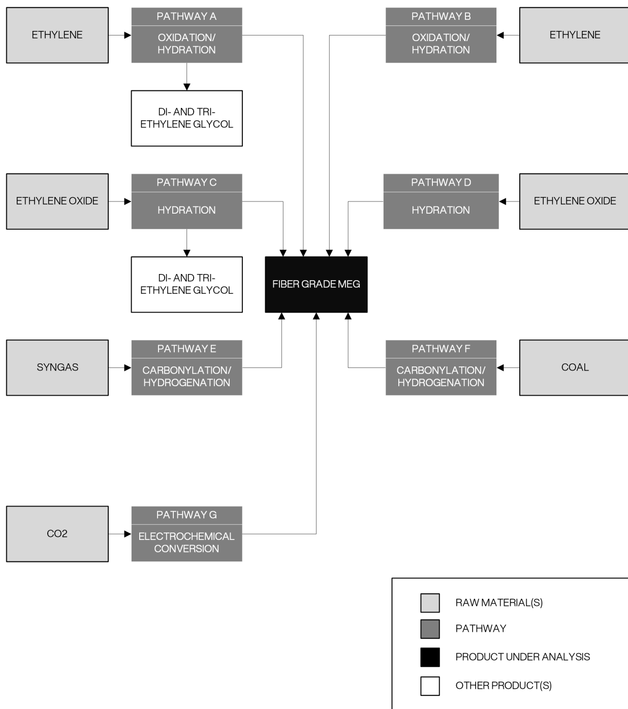
Fiber Grade Ethylene Glycol Production Pathways Diagram
