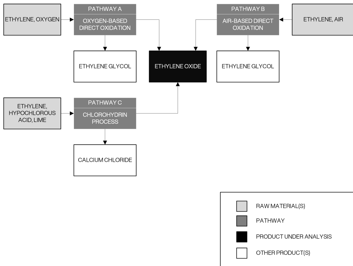
Ethylene Oxide Production Pathways Diagram
