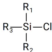
General Chlorosilane Formula
