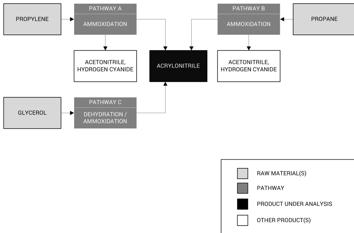
Acrylonitrile Production Pathways Diagram
