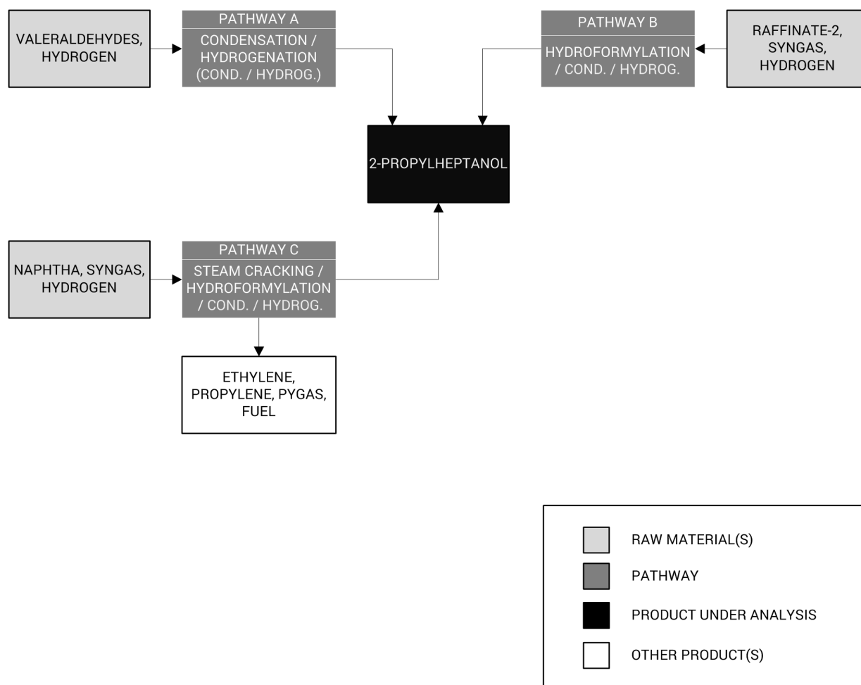
2-Propylheptanol Production Pathways Diagram
