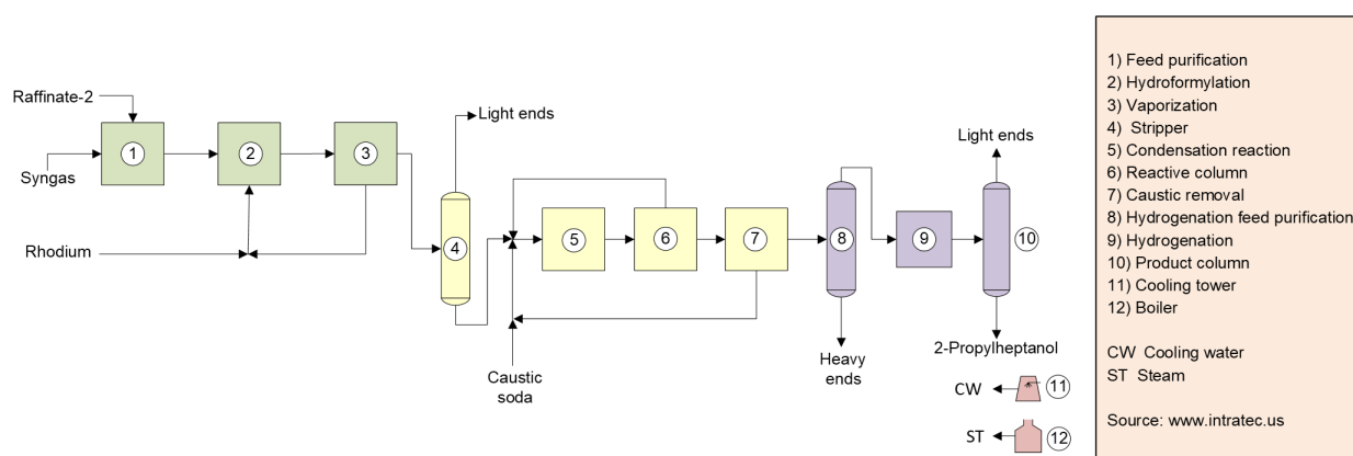
Process Schematic Diagram
