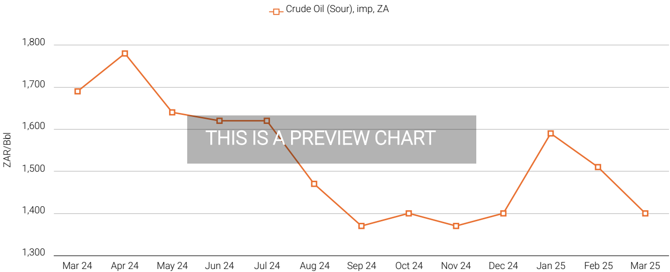
Figure 2.1 South Africa Crude Oil Prices (Mar 24 - Mar 25)
