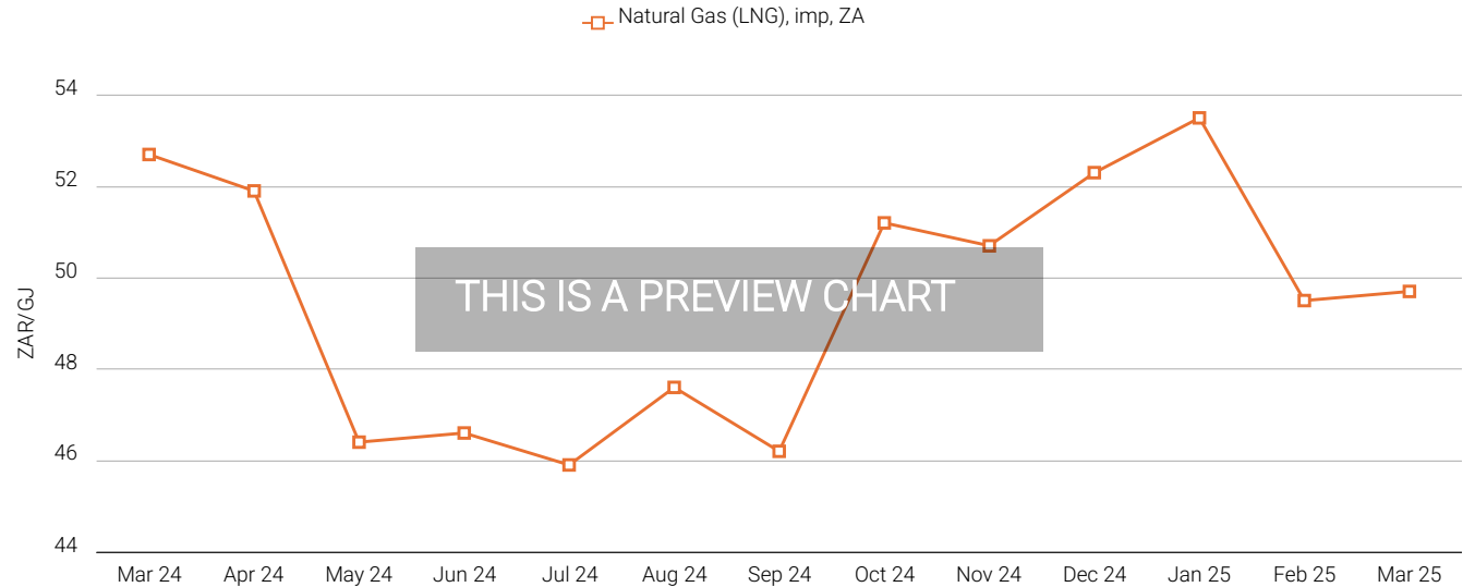
Figure 2.2 South Africa Natural Gas Prices (Mar 24 - Mar 25)
