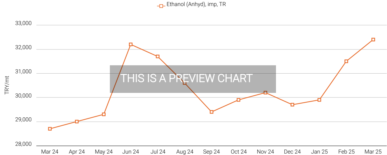
Figure 2.11 Turkey Ethanol Prices (Mar 24 - Mar 25)
