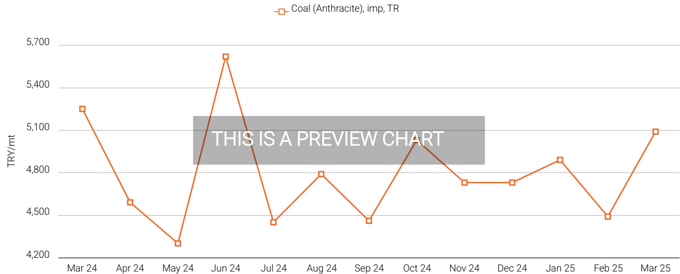
Figure 2.3 Turkey Coal Prices (Mar 24 - Mar 25)
