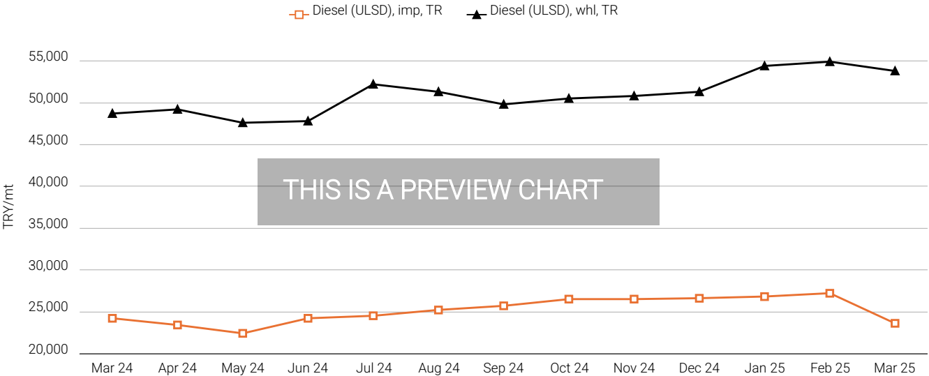
Figure 2.8 Turkey Diesel Prices (Mar 24 - Mar 25)
