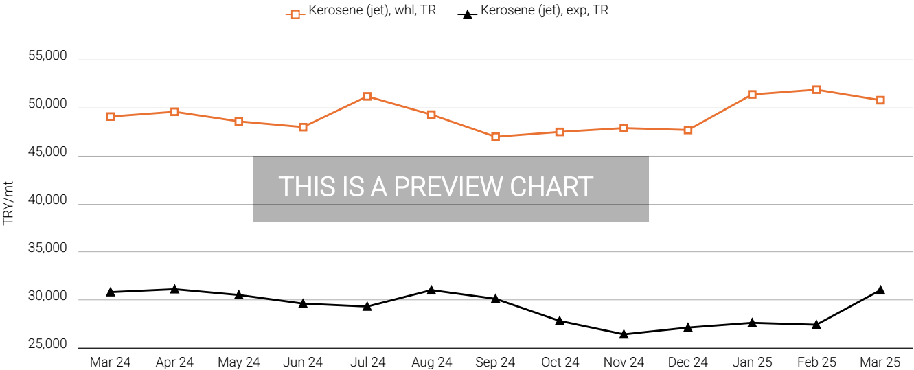
Figure 2.7 Turkey Kerosene Prices (Mar 24 - Mar 25)
