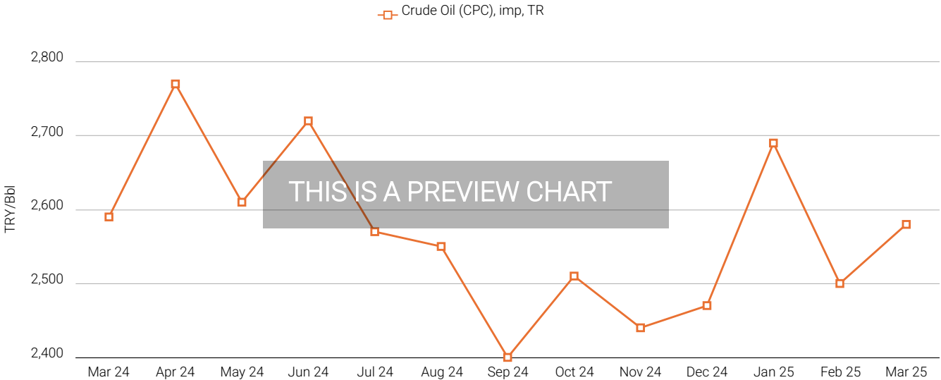
Figure 2.1 Turkey Crude Oil Prices (Mar 24 - Mar 25)
