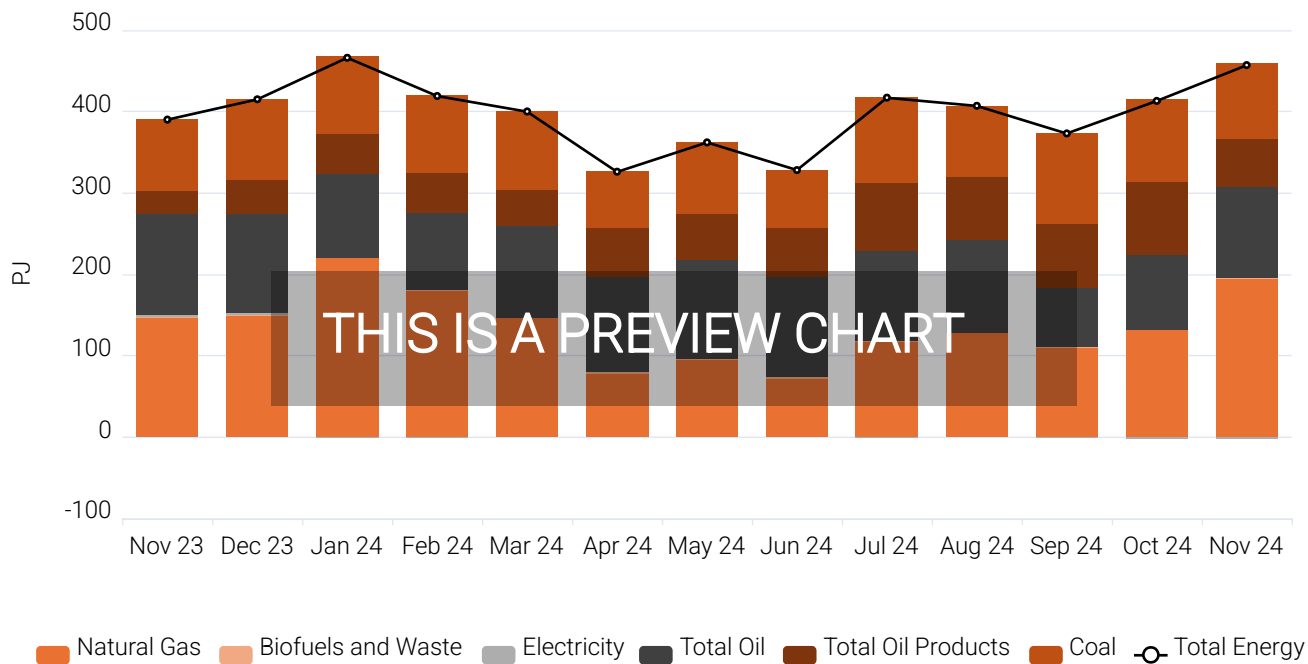
Figure 5.1 Turkey Energy Net Trade, in PJ (Nov 23 - Nov 24)
