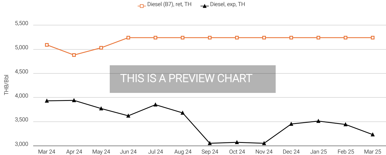
Figure 2.8 Thailand Diesel Prices (Mar 24 - Mar 25)
