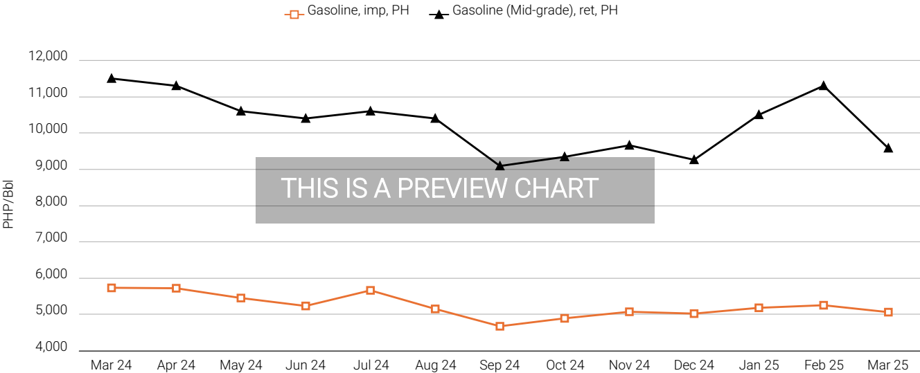
Figure 2.6 Philippines Gasoline Prices (Mar 24 - Mar 25)
