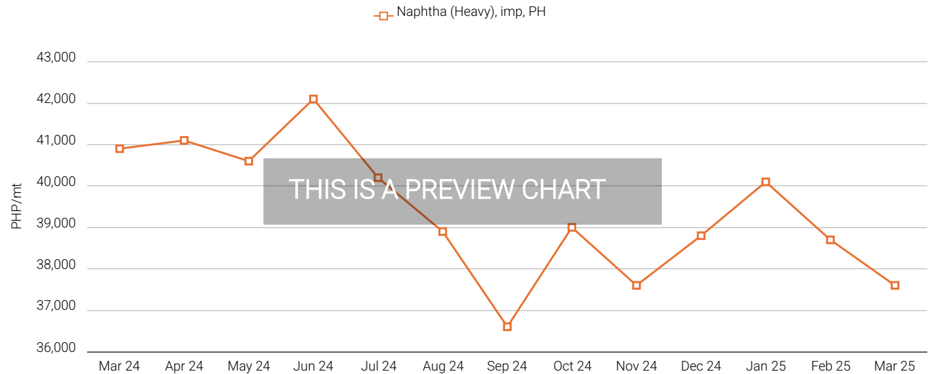
Figure 2.5 Philippines Naphtha Prices (Mar 24 - Mar 25)
