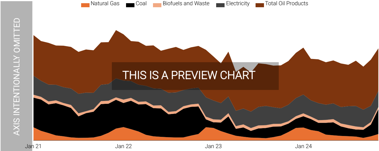
Figure 5.9 South Korea Energy Consumption (Jan 21 - Nov 24)
