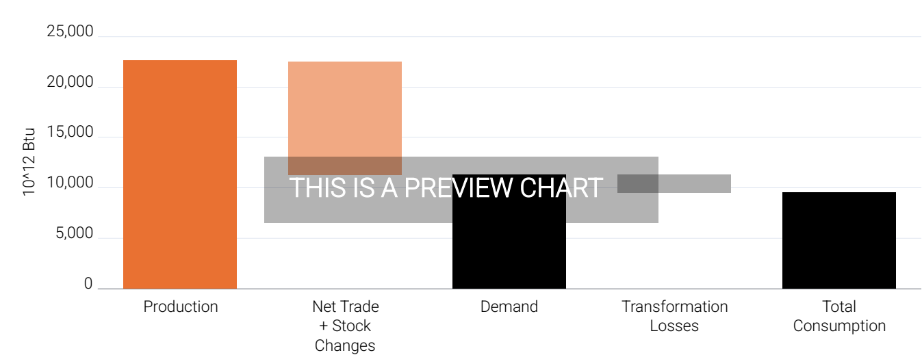
Figure 5.10 Canada Energy Balance (Jan 24 - Nov 24)
