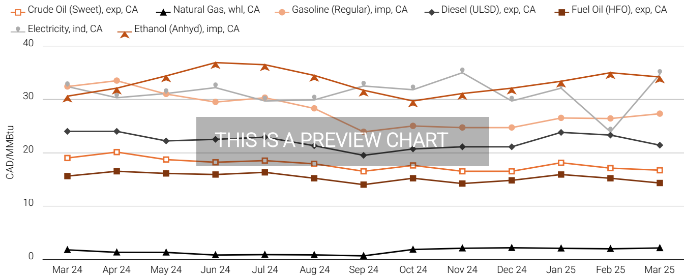
Figure 3.1 Canada Key Energy Prices (Mar 24 - Mar 25)
