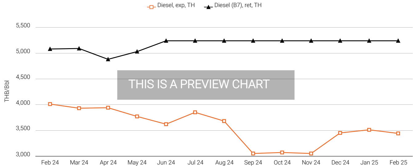
Figure 2.8 Thailand Diesel Prices (Feb 24 - Feb 25)
