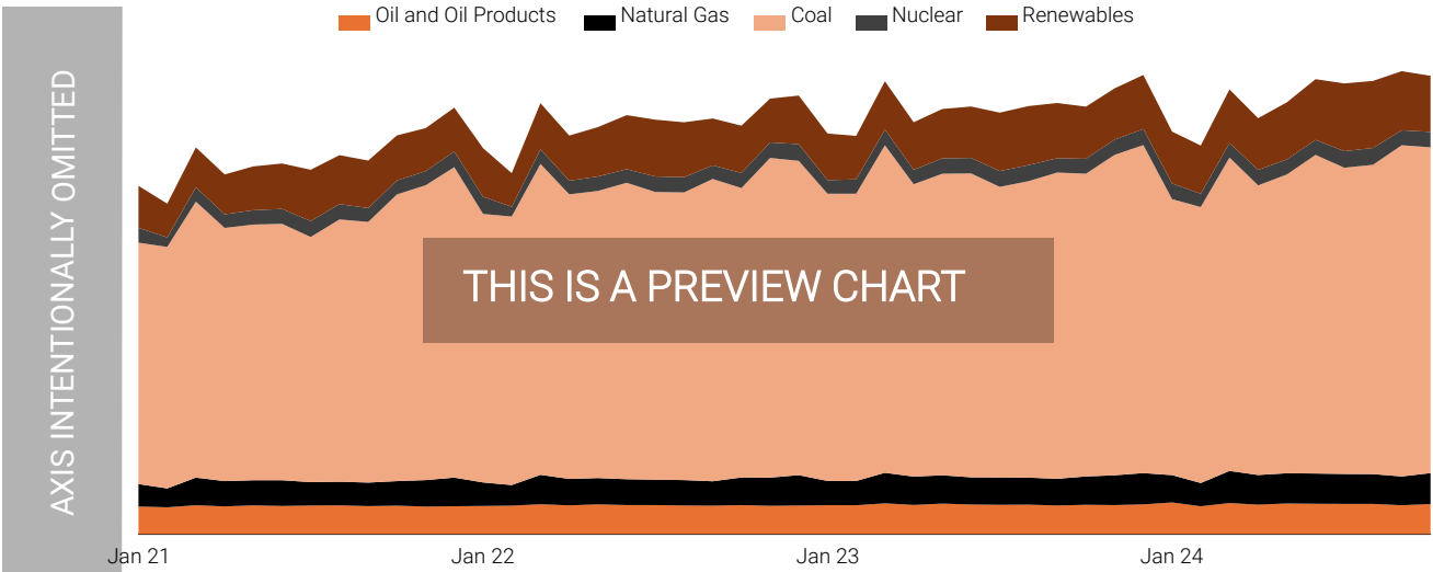
Figure 5.6 China Energy Production (Jan 21 - Oct 24)
