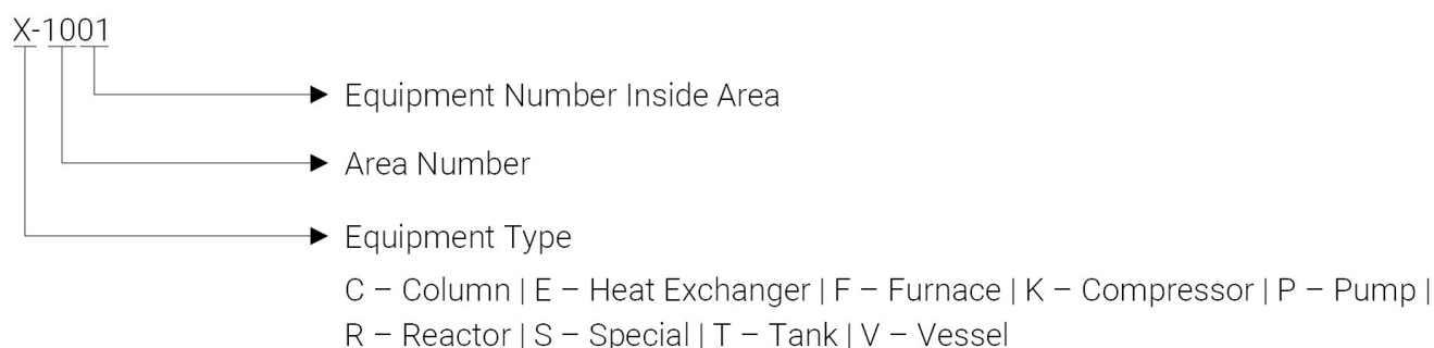
Figure I.1 Convention for Process Equipment Tags
