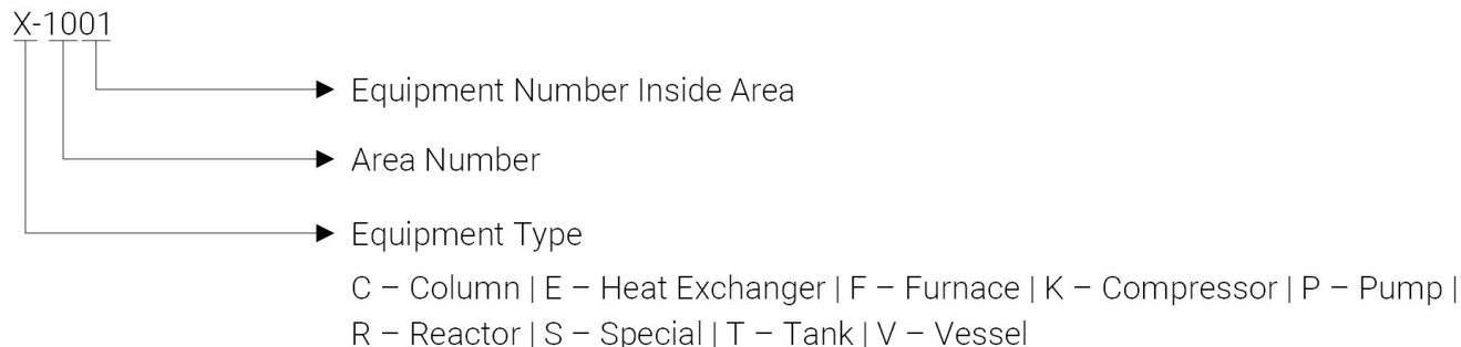
Figure I.1 Convention for Process Equipment Tags
