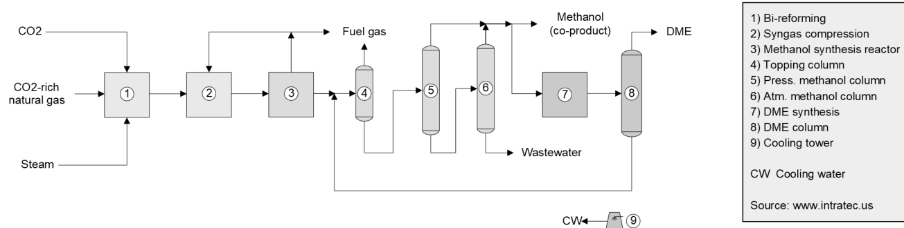
Figure 1.1 Process Schematic Diagram
