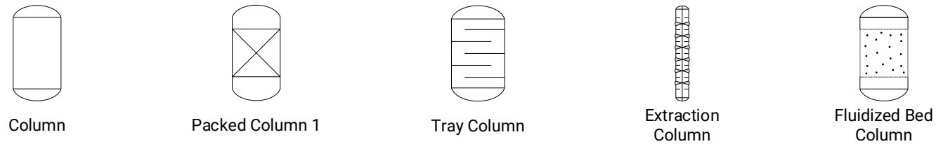
Figure I.6 Equipment Symbols - Columns
