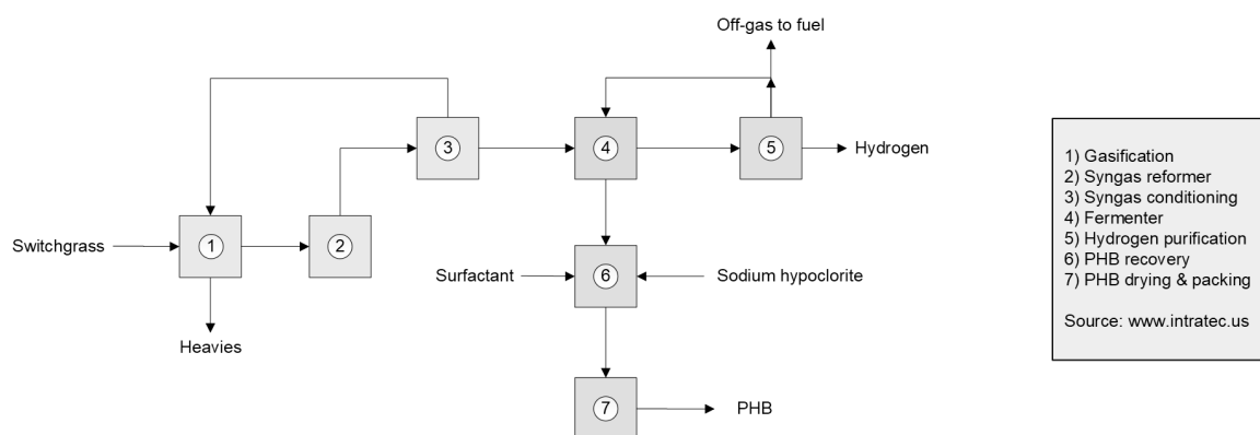
Figure 1.1 Process Schematic Diagram
