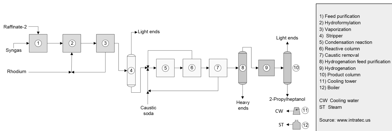
Figure 1.1 Process Schematic Diagram
