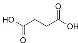
Succinic Acid
