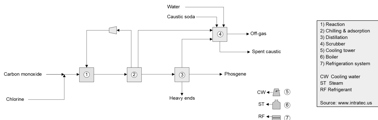
Figure 1.1 Process Schematic Diagram
