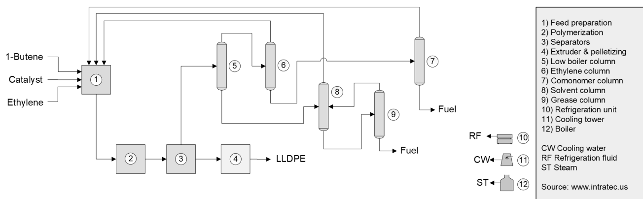
Figure 1.1 Process Schematic Diagram
