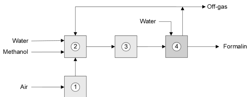
Figure 1.1 Process Schematic Diagram
