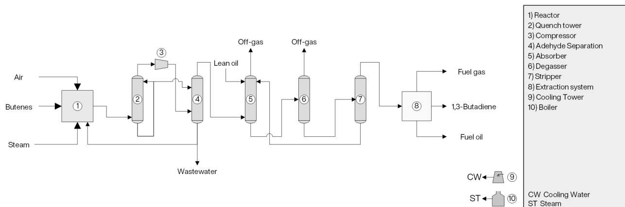
Figure 1.1 Process Schematic Diagram
