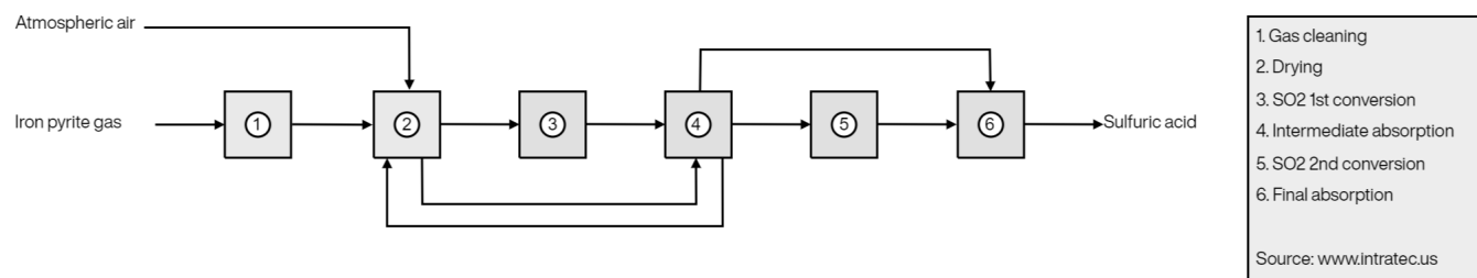
Figure 1.1 Process Schematic Diagram
