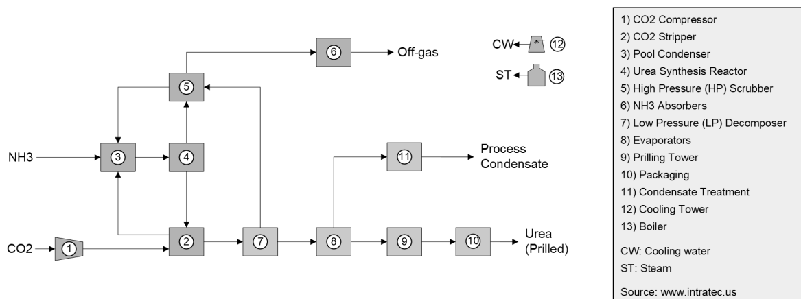
Figure 1.1 Process Schematic Diagram
