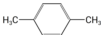
Paraxylene
