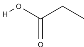
Propionic Acid
