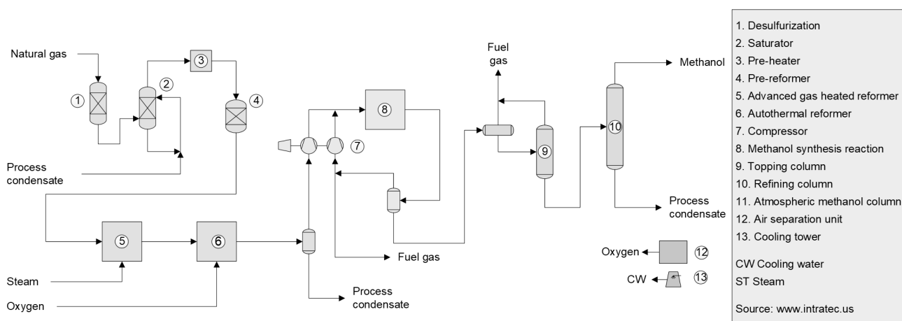
Figure 1.1 Process Schematic Diagram
